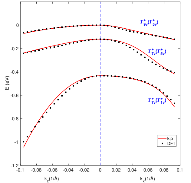
Figure 4. Valence band structure of hex-Ge derived from the 6-band (spinful VBs) fit. The original fitting region k \leq 0.1 \text{ \AA}^{-1} has been preserved to show the deviations, especially for the lower-lying \Gamma_{1v}^+ valance band.
