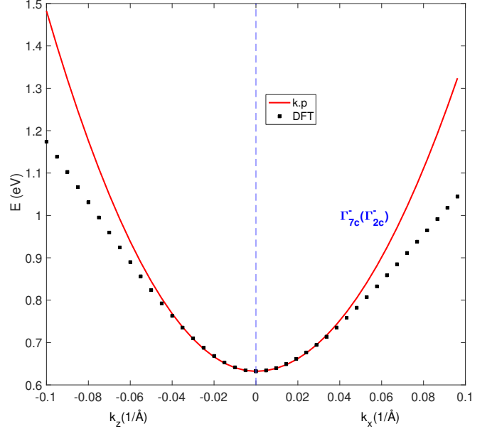
Figure 3. Second-lowest conduction band described by the 2-band (spinful CB+1) low-energy effective Hamiltonian for the 2H-Ge. The original fitting region k \leq 0.1 \text{ \AA}^{-1} has been preserved to show the deviations after 0.05 \text{ \AA}^{-1} .
