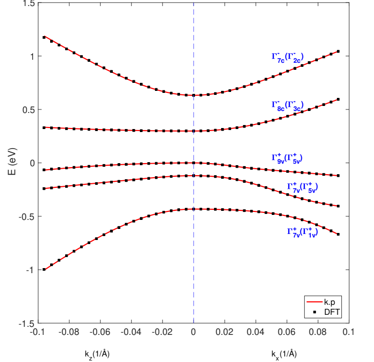
Figure 2. Band structure of hex-Ge around the \Gamma point. \mathbf{k} \cdot \mathbf{p} (solid red lines) fit for the 10 band 2H-Ge, up to the 0.1 \text{ \AA}^{-1} to ab initio (black symbols) for \Gamma \rightarrow A ( k_z ) and \Gamma \rightarrow M ( k_x ) directions. The ordering of the heavy-hole(HH)-light-hole(LH) and crystal-field split-off hole(CH) is due to crystal field splitting being larger than SOC. The combination of inversion and time-reversal symmetry implies that the band structure is doubly degenerate everywhere.
