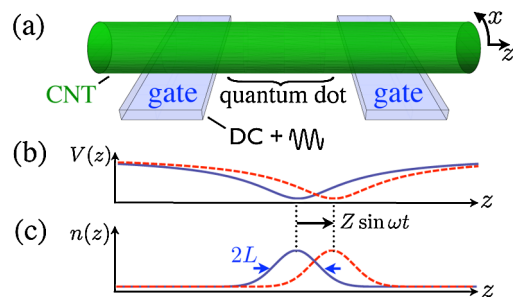
FIG. 1 (color online). Schematic of the valley resonance setup. (a) Two gate electrodes close to the CNT confine an electron to the QD region. (b) The confinement potential V(z) is modulated in time by an ac voltage on the left gate. (c) The modulation of the confinement potential is followed by a displacement of the electron density n(z) . The interplay of this driven motion and disorder induces ac valley mixing leading to the valley resonance effect.
