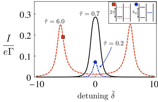
FIG. 3 (color online). Current as a function of the dimensionless detuning \tilde{\delta} = \delta/b_{ac} of the driving frequency from resonance, for different values of the dimensionless tunnel amplitude \tilde{\tau} = \tau/b_{ac} . Inset: Energy diagrams corresponding to the two indicated points of the main plot.
